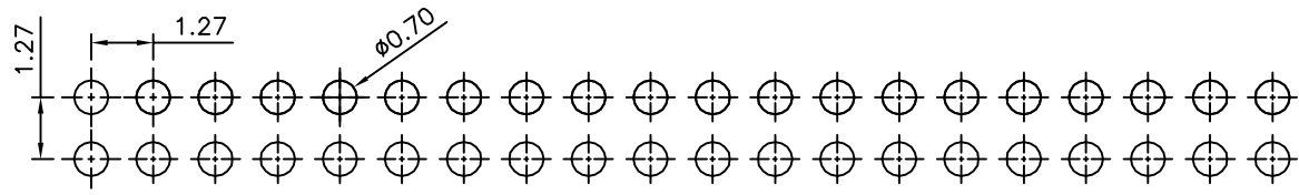
Recommended P.C.B. Layout
