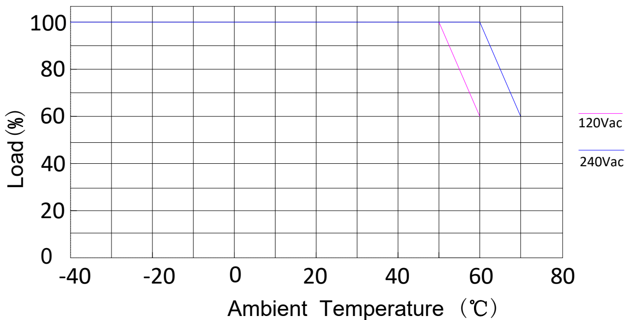
Derating Curve
