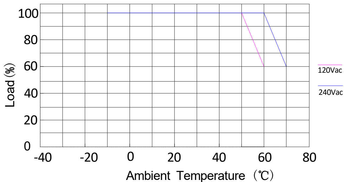
Derating Curve
