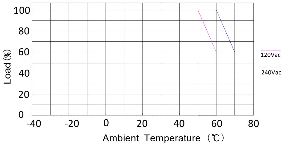
Derating Curve
