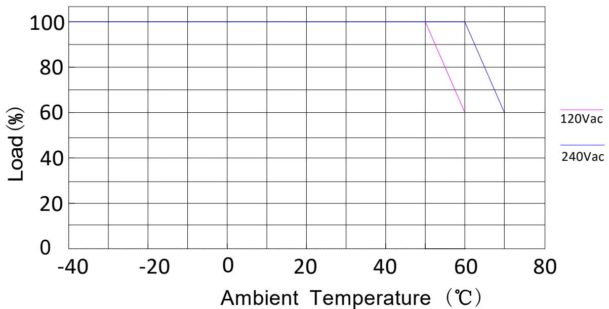
Derating Curve
