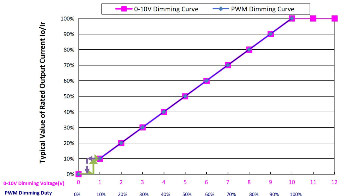
0-10V/PWM Dimming Curve
