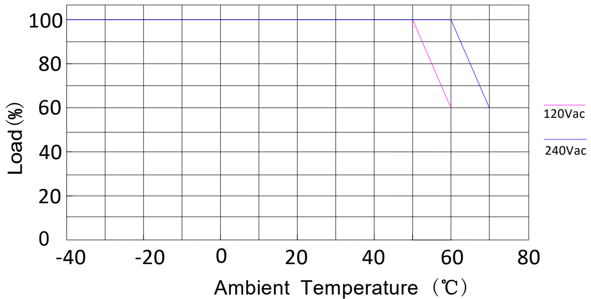
Derating Curve
