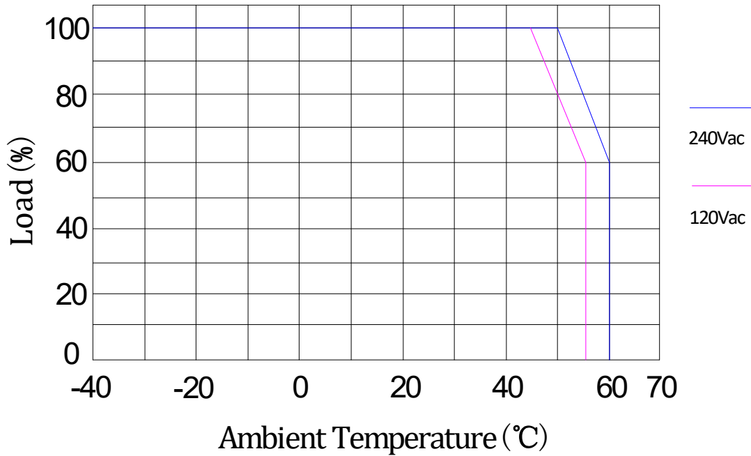
Derating Curve
