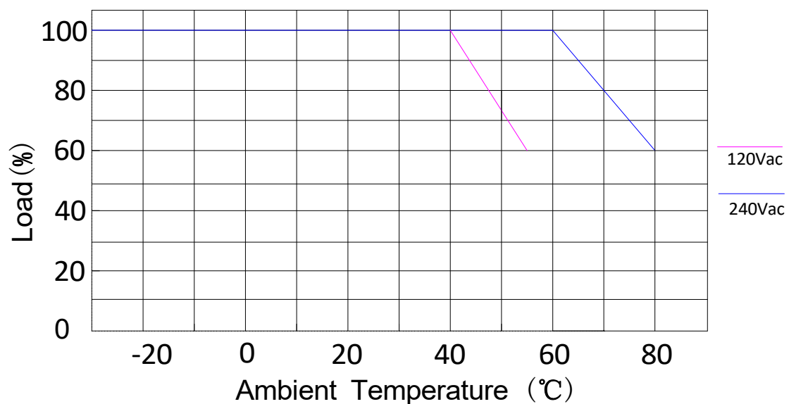
Derating Curve
