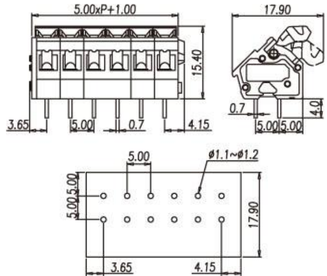
WKA500A-XXP WKA500 - series of terminal blocks A - modification XX - number of Positions (number of Pins/Poles)
