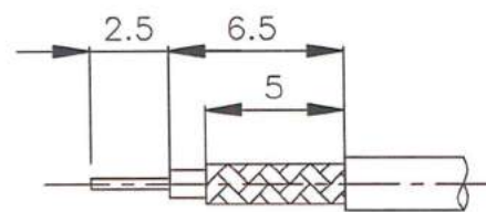
(Recommended Stripping Dimension)
