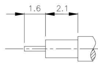
(Recommended Stripping Dimension)
