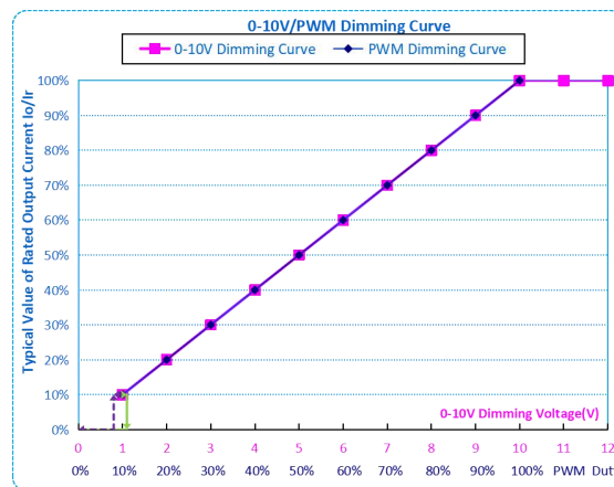
0-10V(5V)/PWM/Rx
