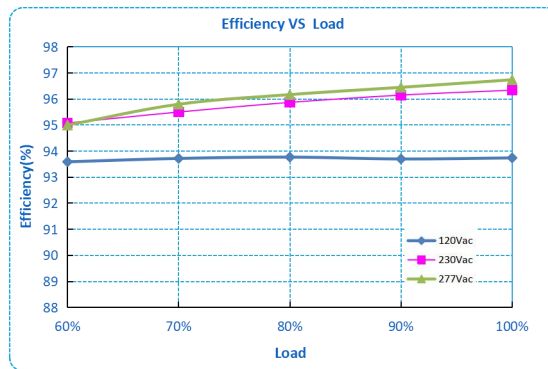
R3-200Y ( I_o=0.83A )
