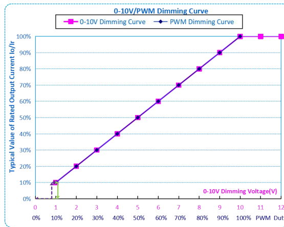
0-10V(5V)/PWM/Rx
