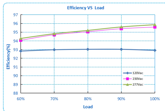
R3-150Y ( I_o=0.62A )
