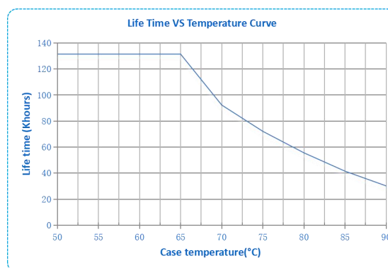
Life Vs. T case
