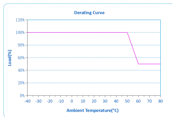
Output power VS Temperature
