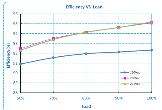
R3-060Y ( I_o=0.24A )
