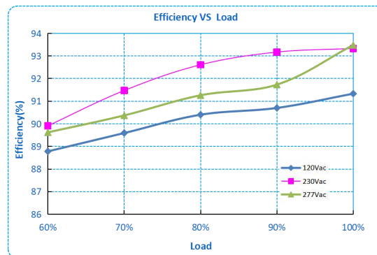
R3-040X ( I_o=0.16A )
