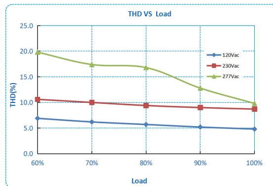
R3-040X Series
