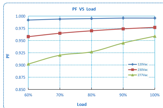
R3-040X Series
