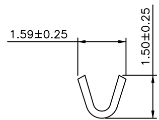
△ B-B Section
