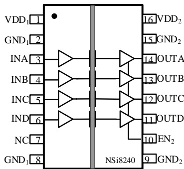
Figure 1.1 NSi8240W Package
