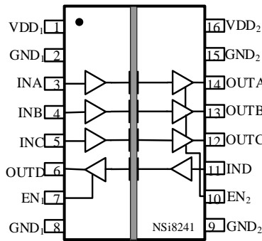
Figure 1.2 NSi8241W Package
