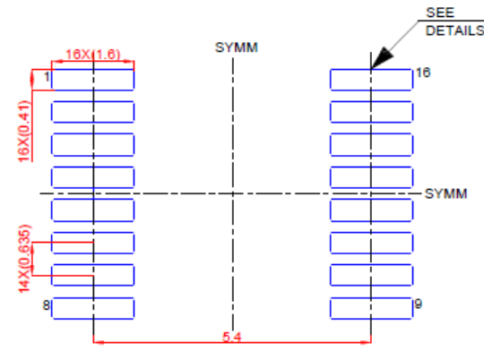
Figure 9.5 SSOP16 Package Shape and Dimension in millimeters
