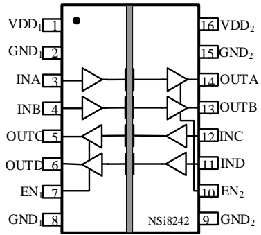
Figure 1.3 NSi8242W Package
