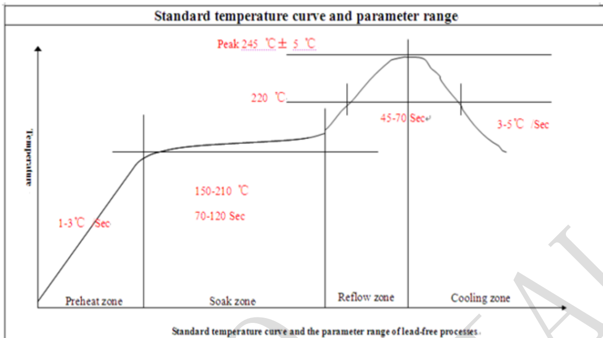
Figure 11 The Ramp-Soak-Spike reflow profile of N20
