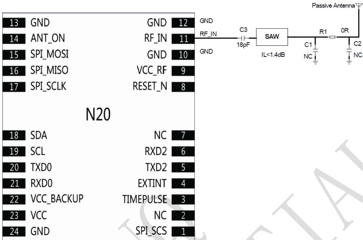
Figure 7 N20 passive antenna designs(with external saw)
