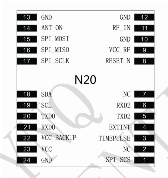
Figure 2 N20 pin out diagram (Top view)
