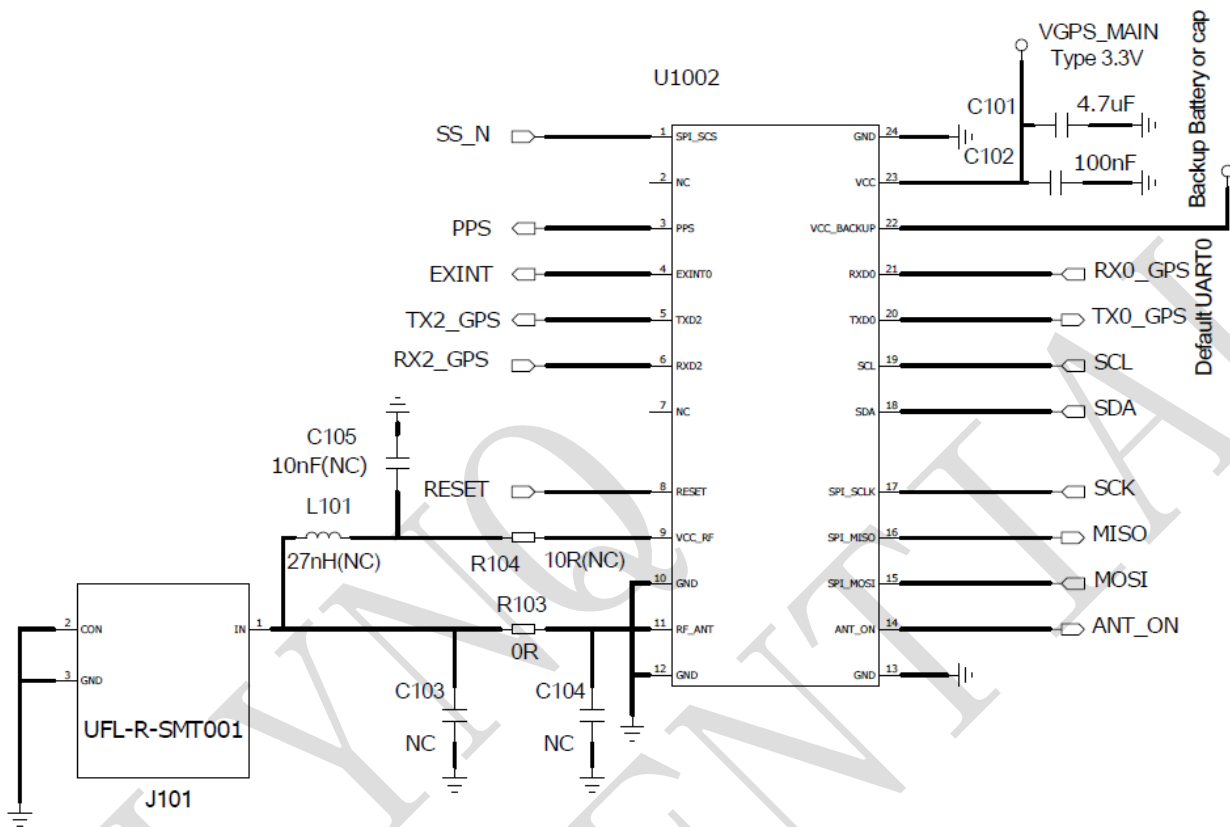
Figure 12 Application schematics
