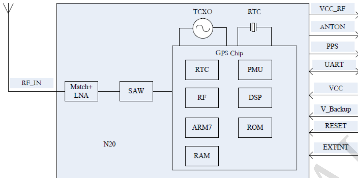
Figure 1 N20 functional diagram
