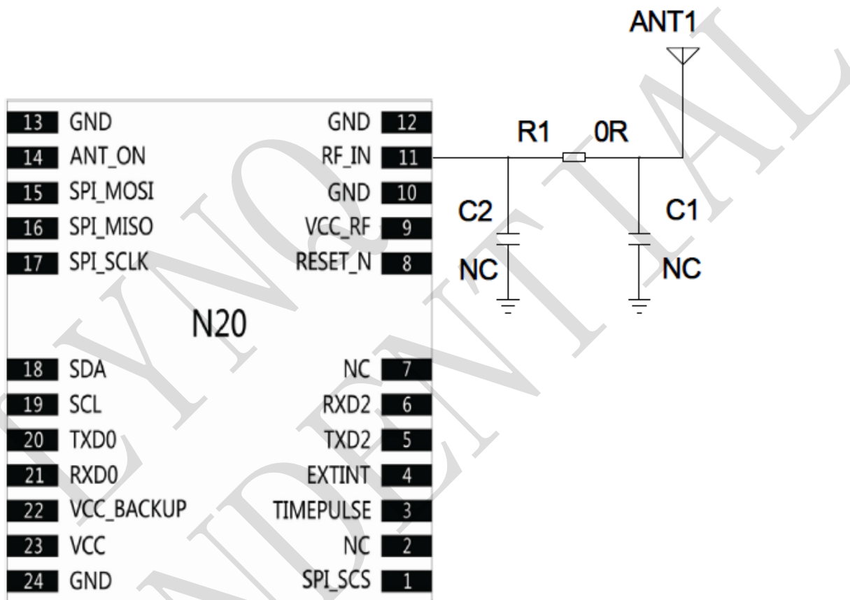
Figure 6 N20 passive antenna designs
