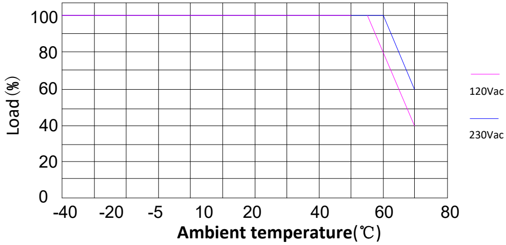
Derating curve
