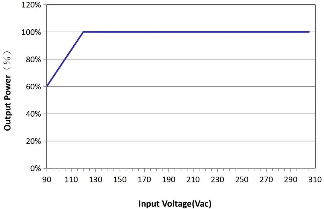
Output Power VS Input Voltage Curve
