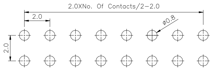
Recommended P.C.B. Layout(Top View) (PCB Board Tolerance±0.05)
