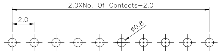
Recommended P.C.Board Layout(Top View) (PCB Board Tolerance±0.05)
