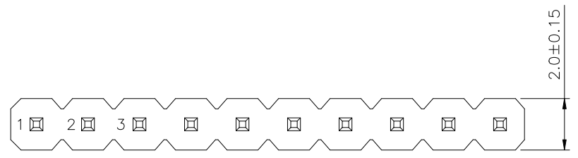
Recommended P.C.Board Layout(Top View) (PCB Board Tolerance±0.05)
