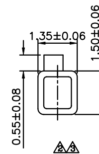
Section B-B
