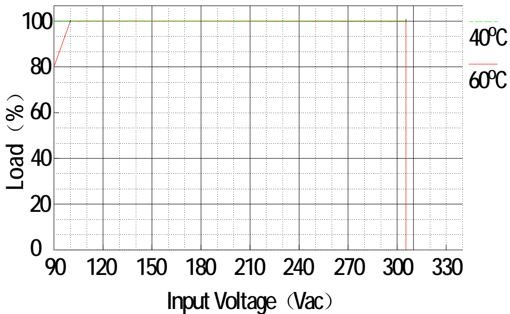
Input voltage vs. Load Curve
