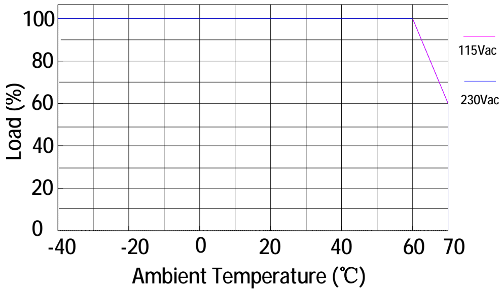
Temperature vs. Load Curve
