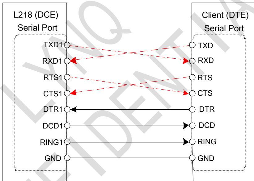
Figure 3-18: Full-featured serial connection
