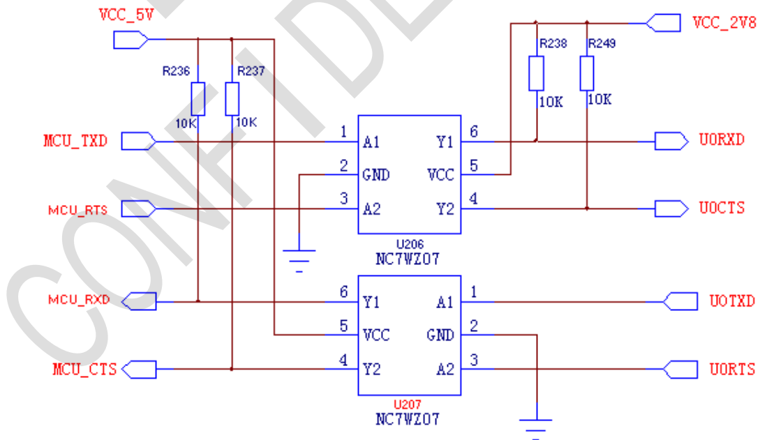
Figure 3-24: Chip level matching (Reference circuit)
