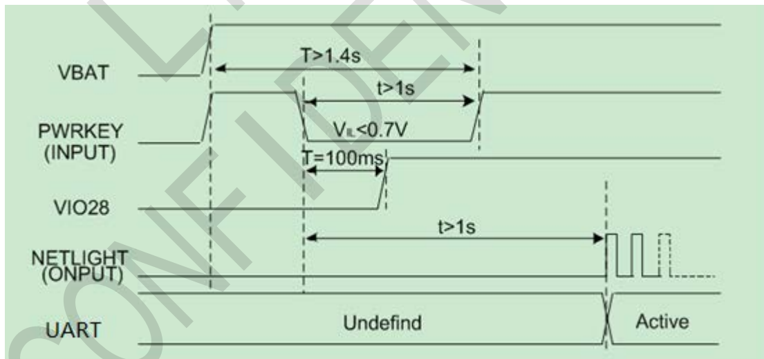
Figure 3-8: Boot sequence
