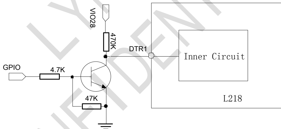
Figure 3-12: DTR circuit
