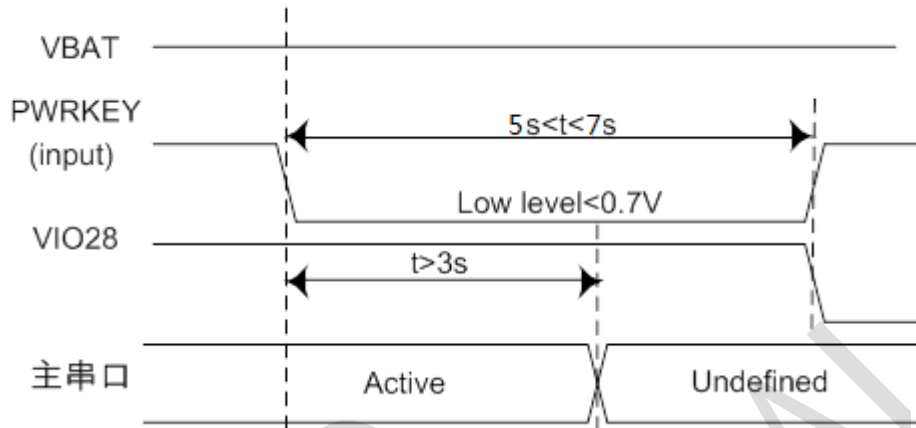
Figure 3-9 Shutdown sequence
