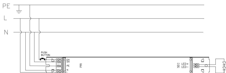
Fig. B: Push Dimming
