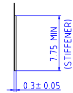
APPLICABLE FPC THICKNESS
