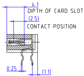
ODD PIN POSITION
