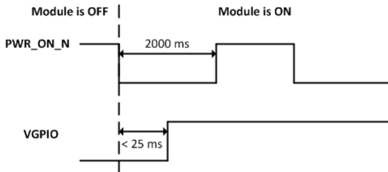
Figure 22. PWR_ON_N Sequence with VGPI0 Information
