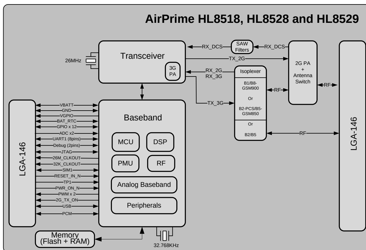
Figure 1. Architecture Overview
