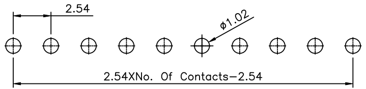
Recommended P.C.B. Layout(Top View) (PCB Board Tolerance±0.05)
