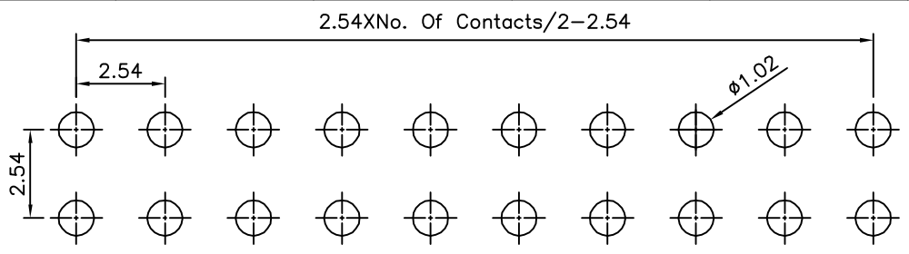
Recommended P.C.B. Layout(Top View) (PCB Board Tolerance±0.05)
