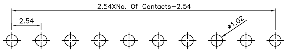
Recommended P.C.B. Layout(Top View) (PCB Board Tolerance±0.05)
