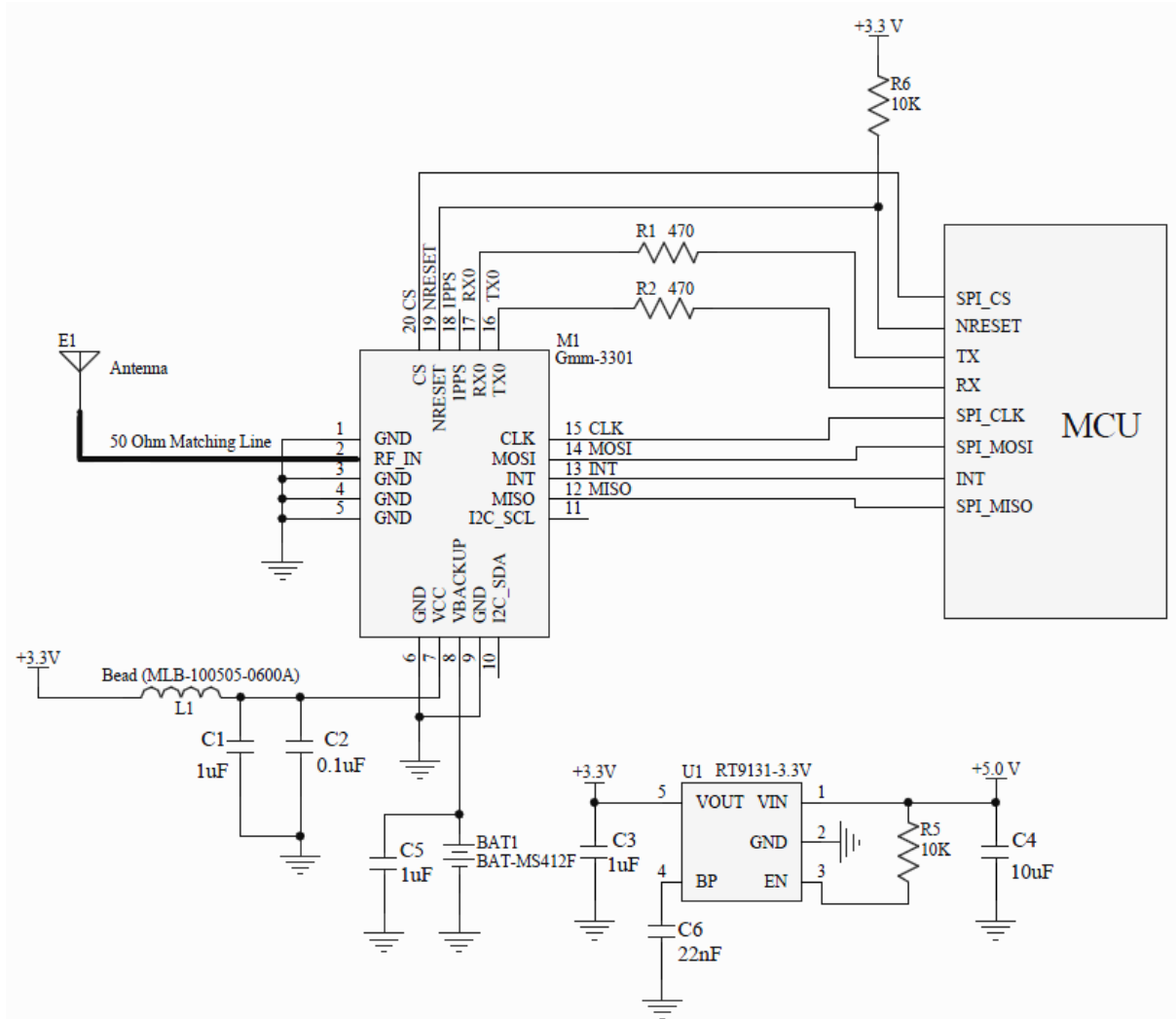
Fig. 4.3 UART+SPI application
