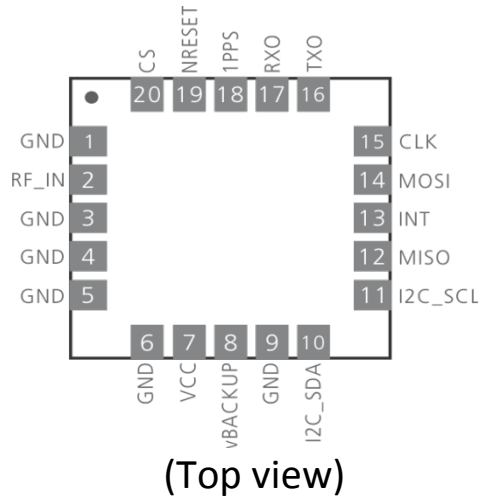
Fig. 2.3 Pin Configuration
