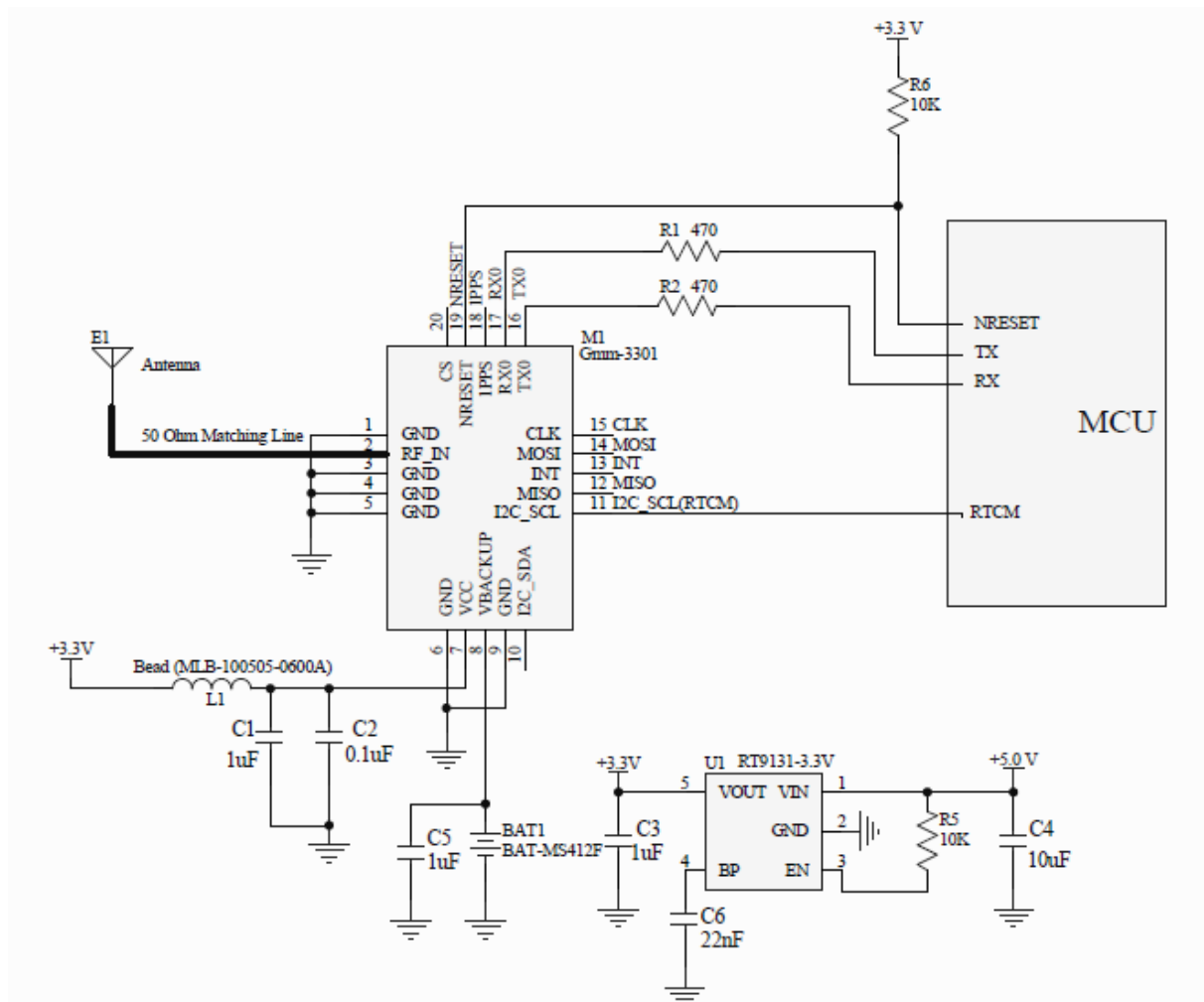
Fig. 4.1 UART+RTCM application
