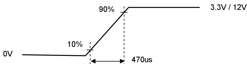
VDD & VLED rising time
