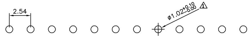
Recommended P.C.B Layout(Top Side) (PCB Board Tolerance±0.05)
