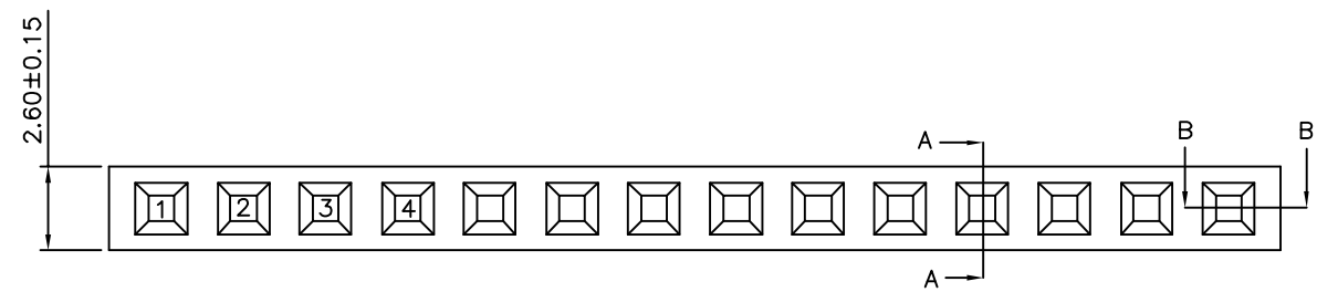
Recommended P.C.B Layout(Top Side) (PCB Board Tolerance±0.05)
