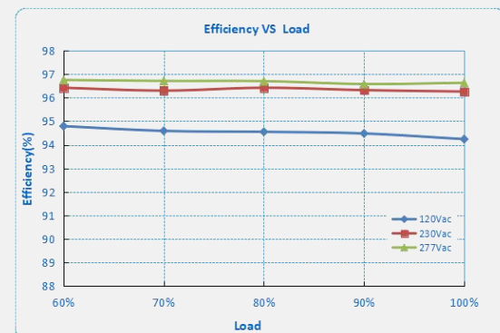
F2-240D-343 ( I_o=0.7A )
