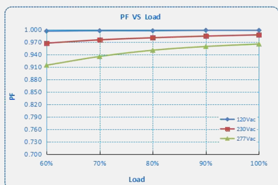
F2-240D Series
