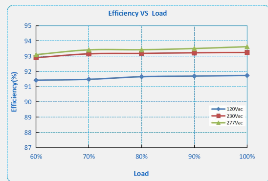
F2-200X-286 ( I_o=0.7A )
