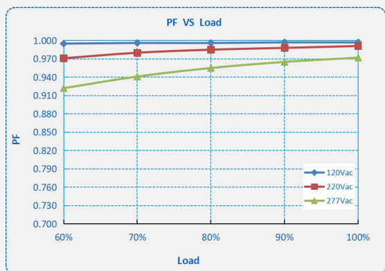
F2-200D Series
