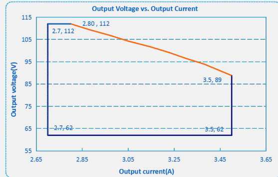
F1E-320X-112
