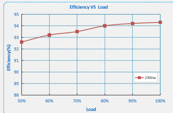
F1E-320X-112 ( I_o=2.8A )
