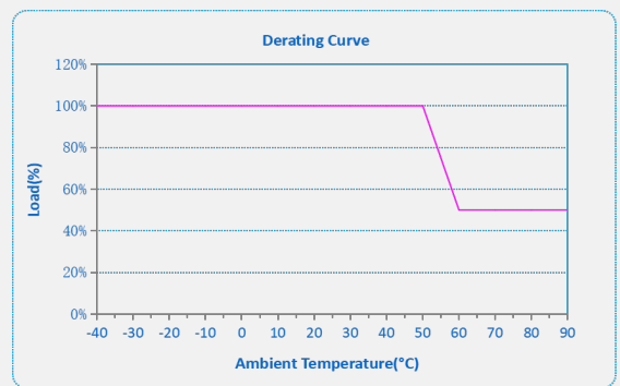
Output Power Vs. T a
