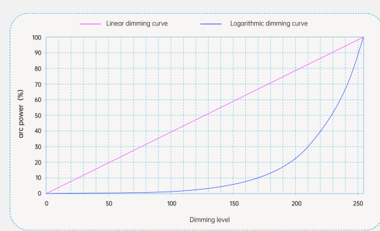
DALI-2 Dimming Curve
