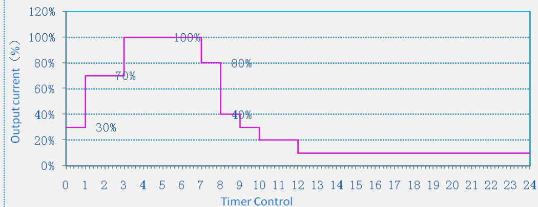
Timer Dimming Diagrammatic
