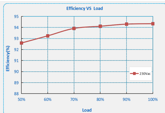
F1E-150X-143R ( I_o=1.05A )
