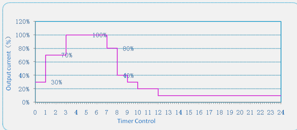
Timer Dimming Diagrammatic
