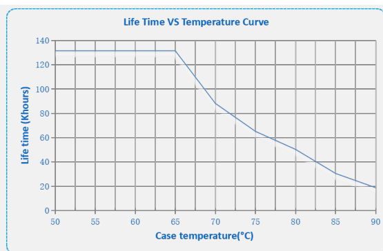
Life Vs. T case
