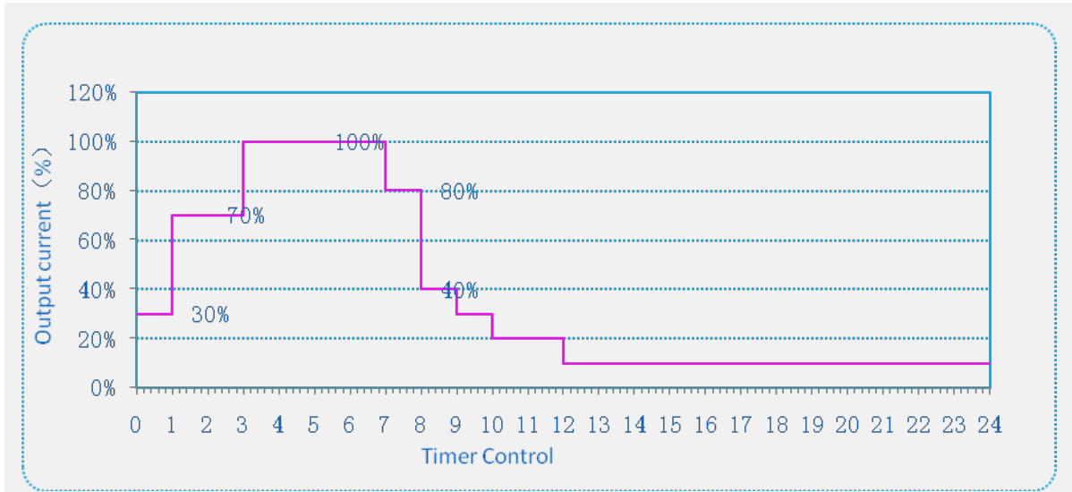
Timer Dimming Diagrammatic
