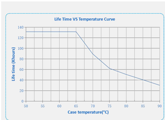
Life Vs. T case
