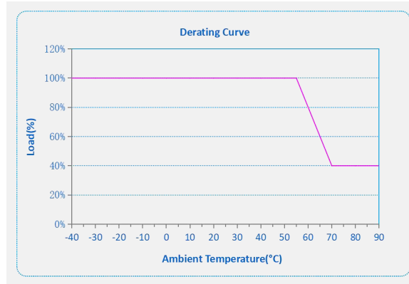
Output Power Vs. Ta
