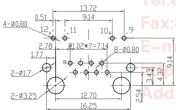
PCB LAYOUT THICKNESS=1.6mm LED Voltage=2.6V
