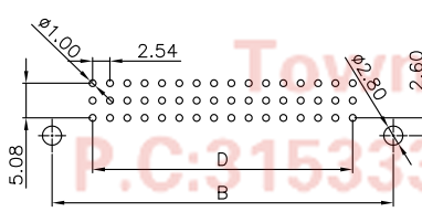
RECOMMEND PCB LAYOUT(FOR MALE) THICKNESS=1.6±0.10mm
