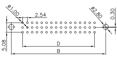
RECOMMEND PCB LAYOUT(FOR FEMALE) THICKNESS=1.6±0.10mm
