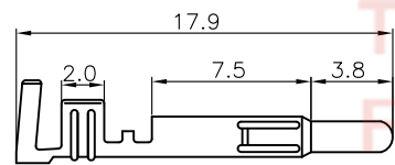
Male TERMINAL
