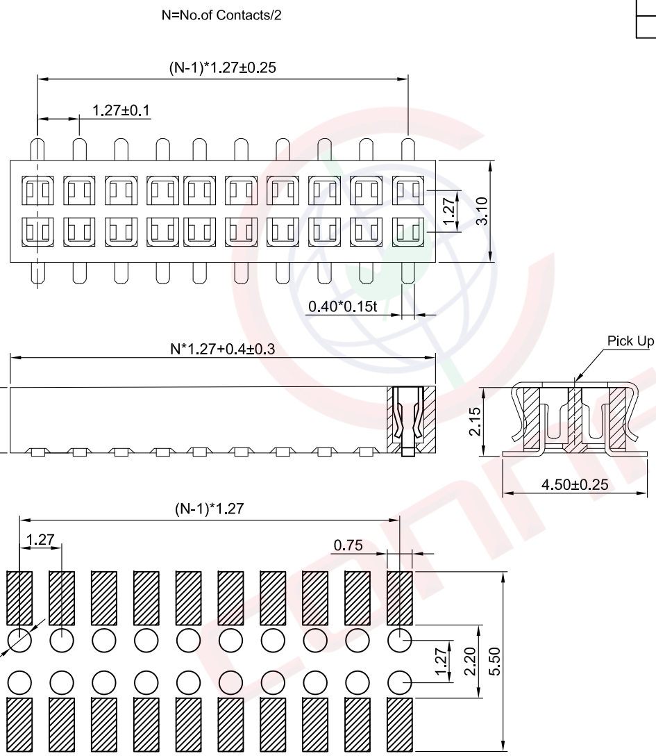
RECOMMEND PCB LAYOUT
