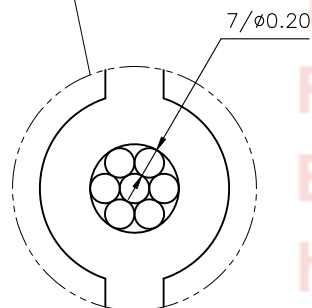
Stranded Type DETAIL (SCALE 8:1)
