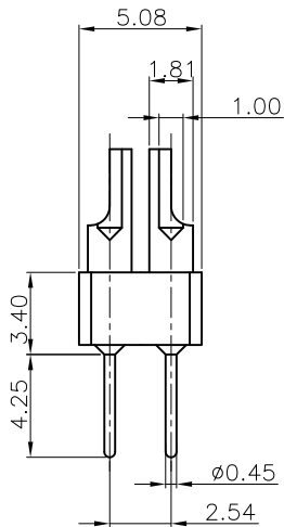
Dual ROW
