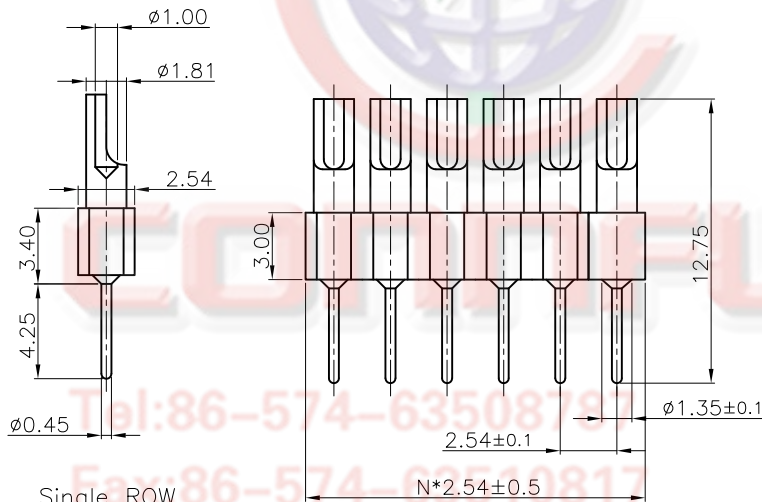
Single ROW
